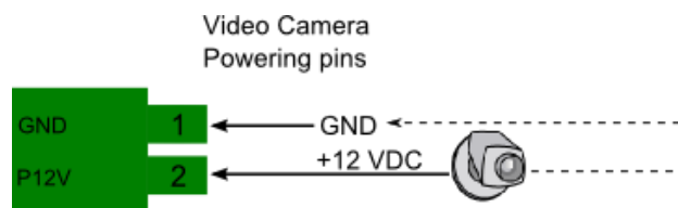
Figure 2-4 12VDC Video Camera Power Connector
