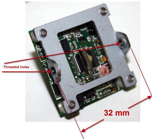
Figure 2-2 PIN-hole video camera bracket (Example)
