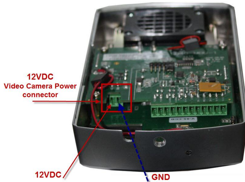
Figure 2-4 12VDC Video Camera Power Connector
