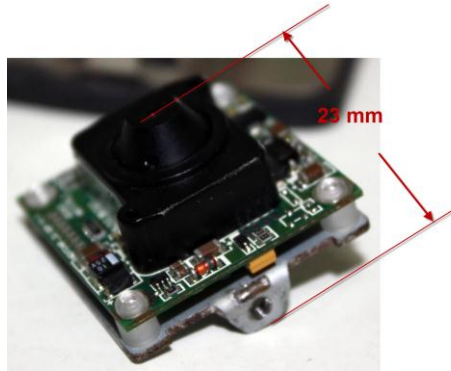
Figure 1-3 PIN-hole analog video camera heights is 23 mm (Example)
