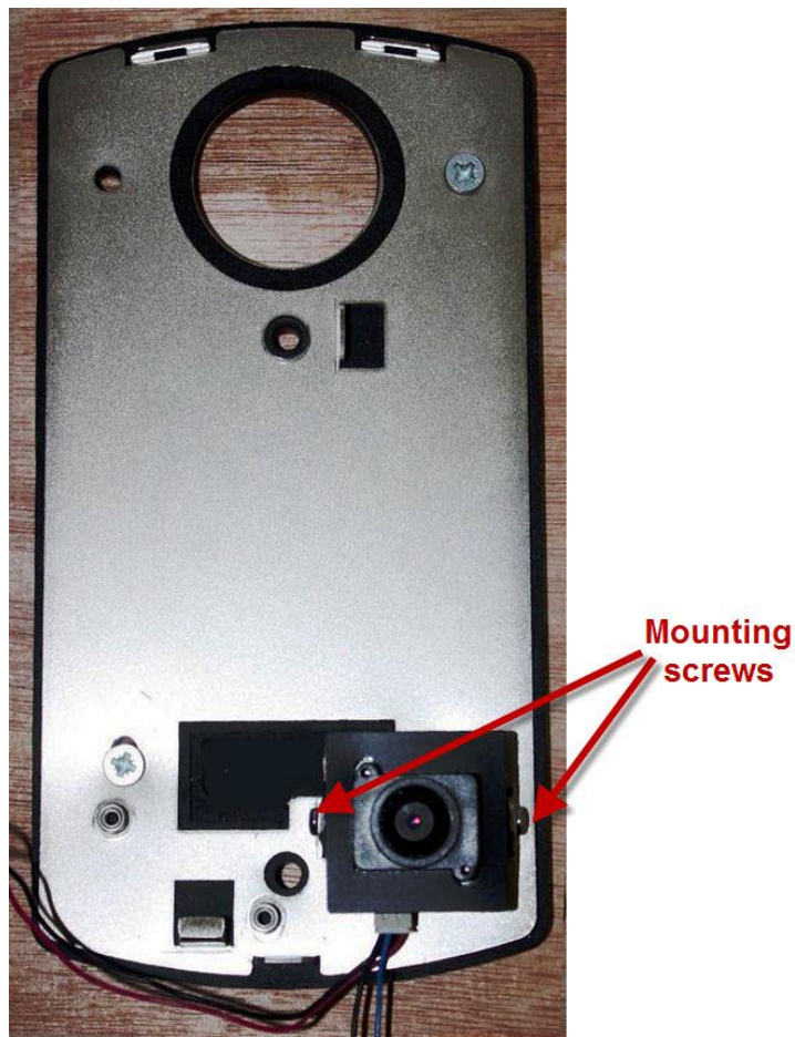
Figure 2-3 Installed video camera
